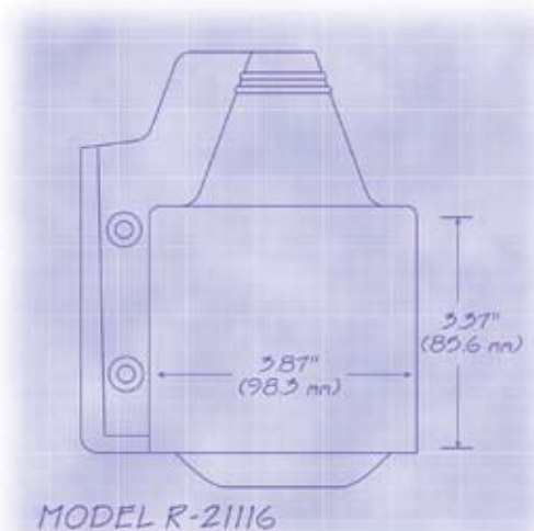
Model R-21116 RUP Bushing Cover & RUP Stinger Cover Combination
